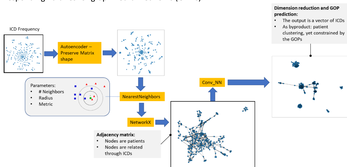
Figure 5 Algorithm's architecture
